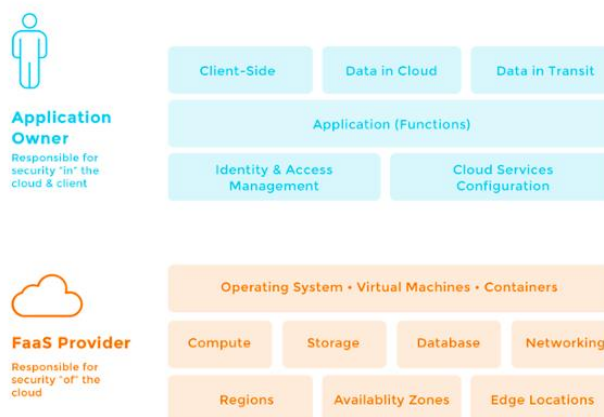
Figure 10: Serverless Security Using the Shared Model [32]
