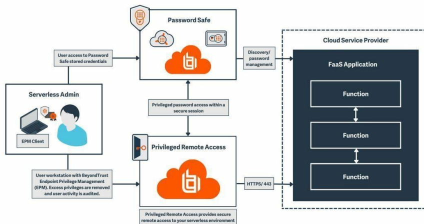
Figure 9: Serverless Security Practices [30]
