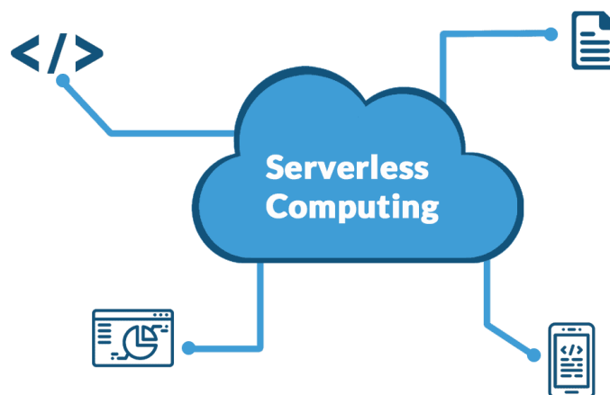
Figure 1: Serverless Computing [2]
